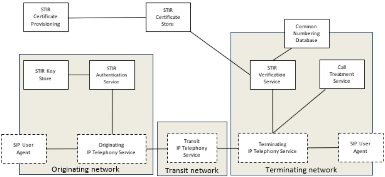
Figure 5.1a: UK STIR architecture – UK origination
